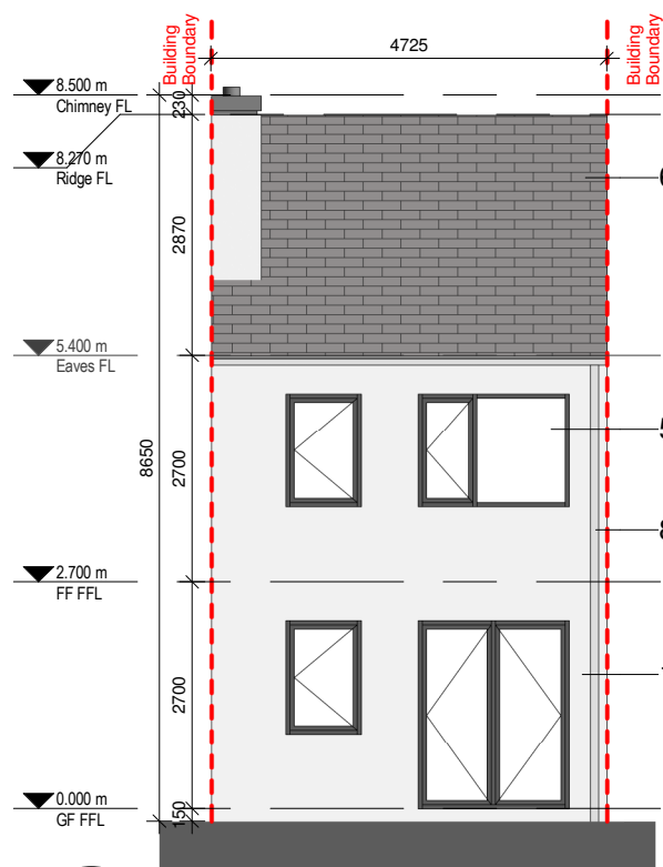
5 Rear Elevation 1 : 100 @ A3
