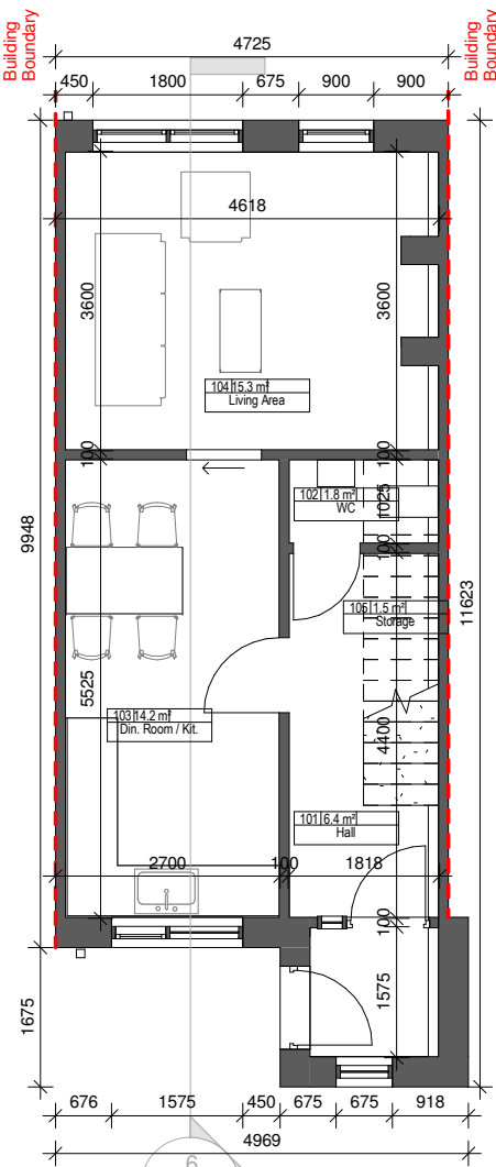
1 Ground Floor Plan 1 : 100 @ A3
