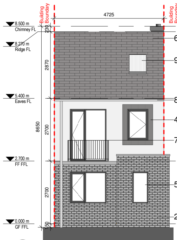
4 Front Elevation 1 : 100 @ A3
