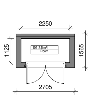
1 Shed Floor Plan 1 : 100 @ A3
