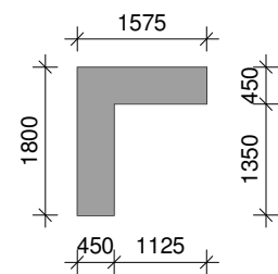
5 Bin Store Plan 1 : 100 @ A3
