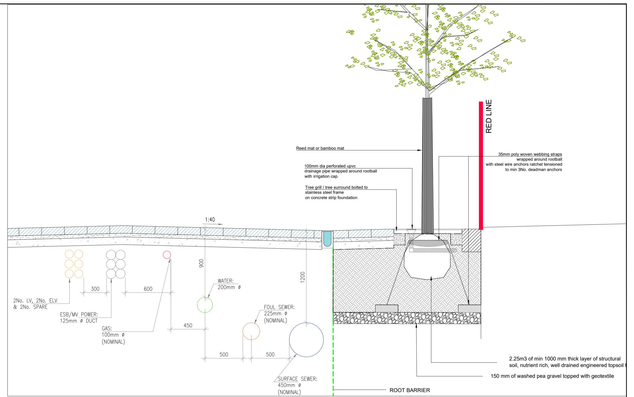
FEATURE TREES TO EASTERN STREET, 1: 25
