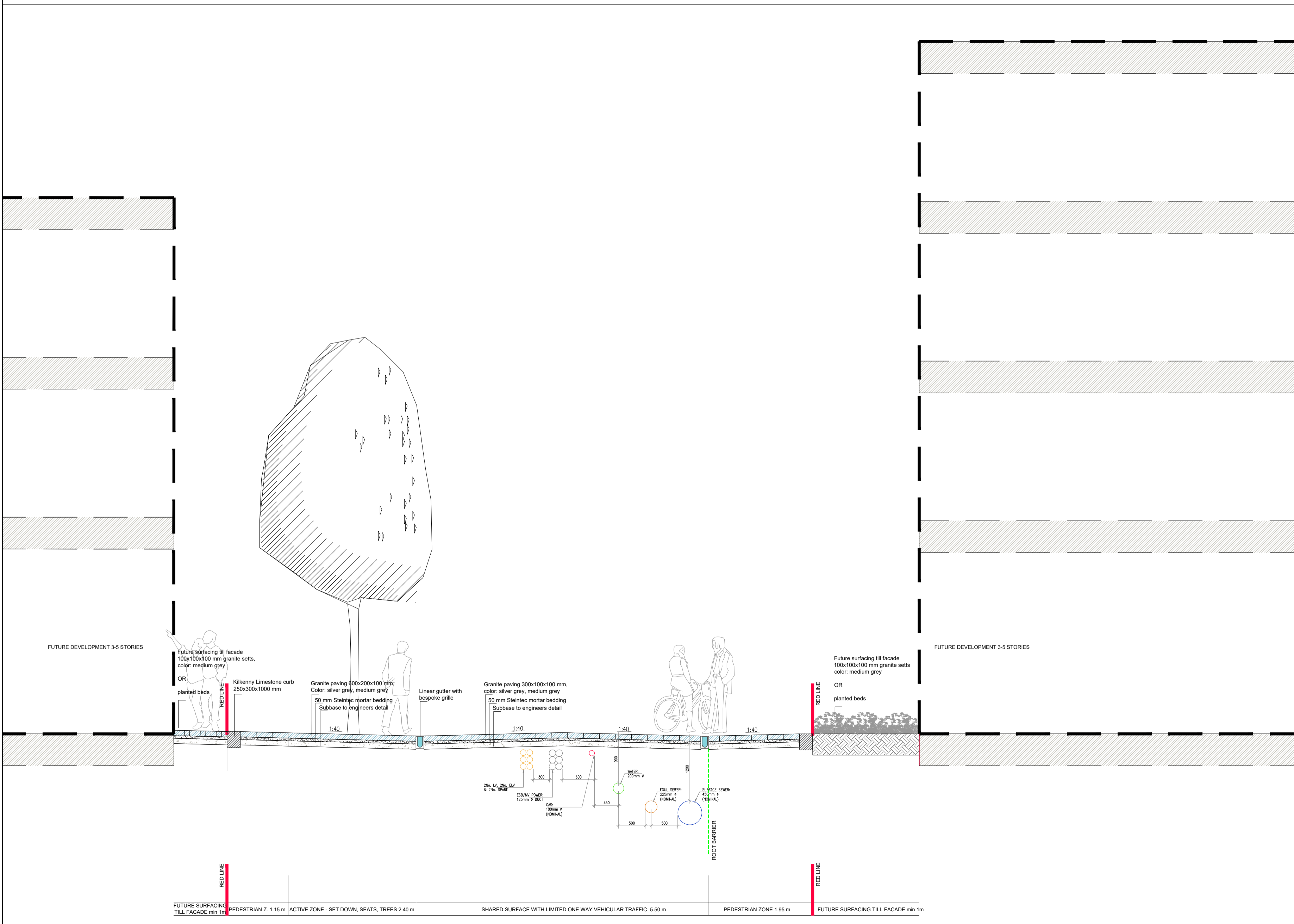
STREET TYPICAL SECTION, 1: 50
