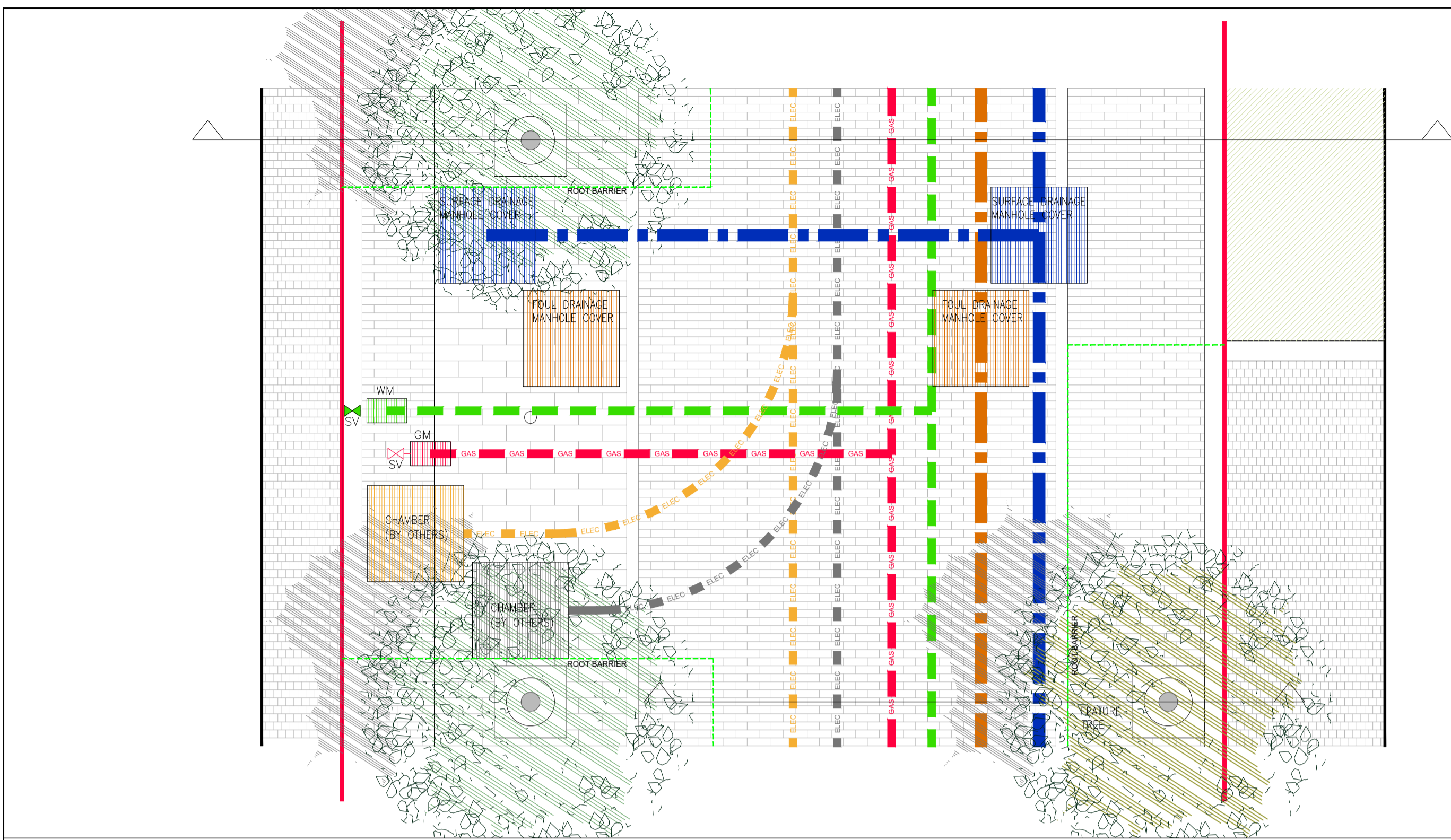
STREET TYPICAL LAYOUT, 1: 50
