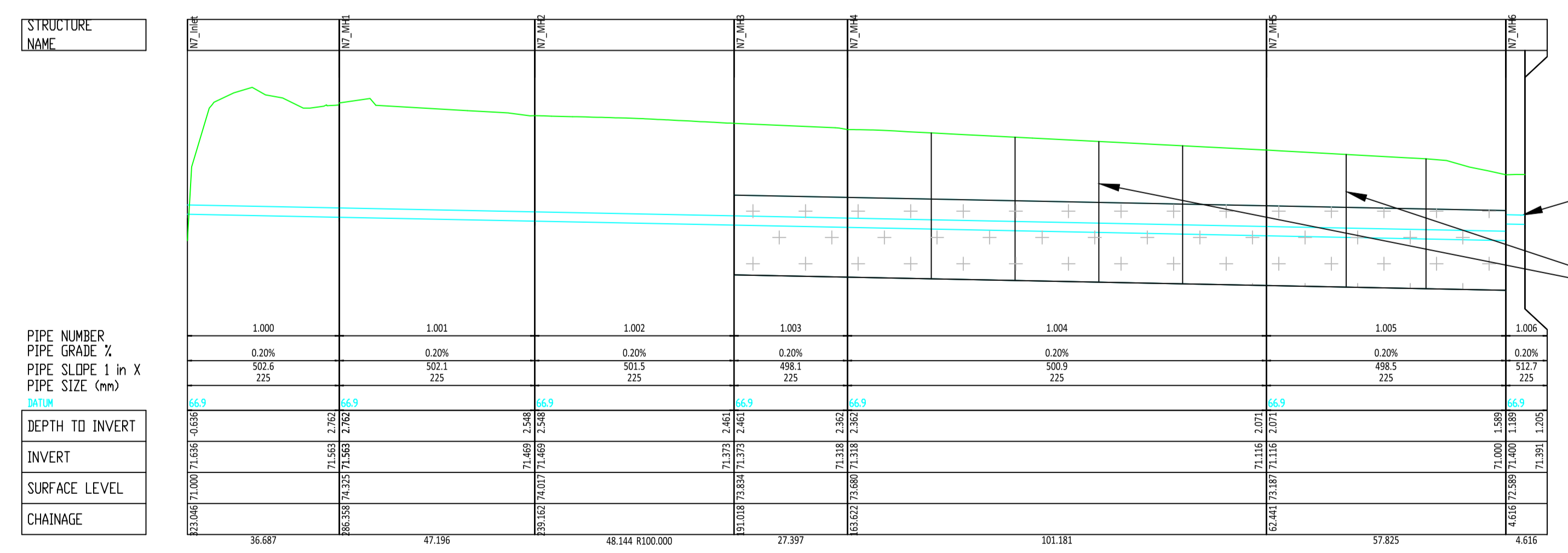
Longsection Drainage Network 7 From Attenuation Pond to Overflow From Infiltration Trench
