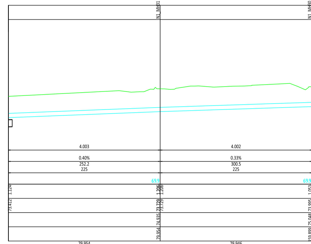
Longsection Drainage Network 1 (Pipe-run 4.000 to 4.003)
