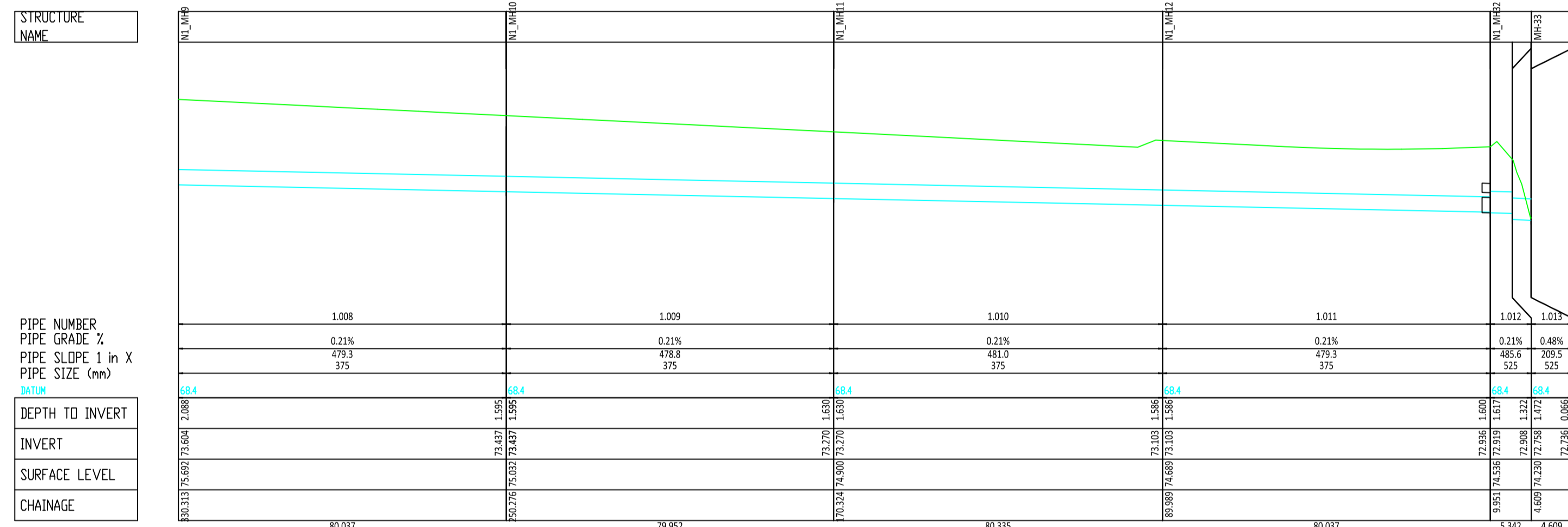
Longsection Drainage Network 1 (Pipe-run 1.008 to 1.013)
