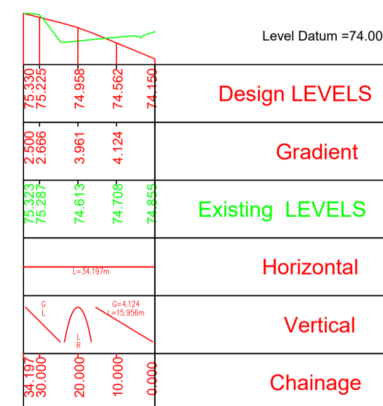
Long-section along Centreline of Direct Access No. 2 Public
