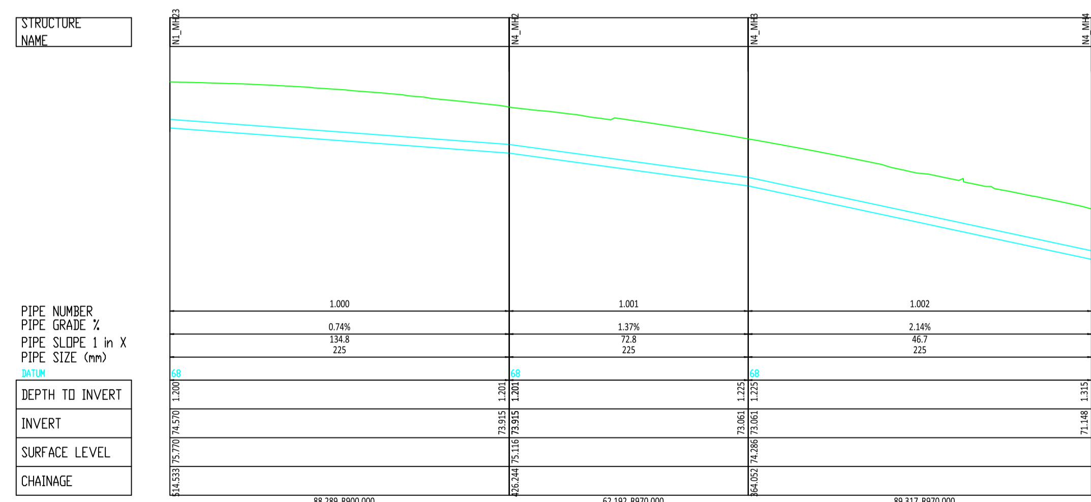
Longsection Drainage Network 4 (Pipe-run 1.000 to Pipe-run 1.007)
