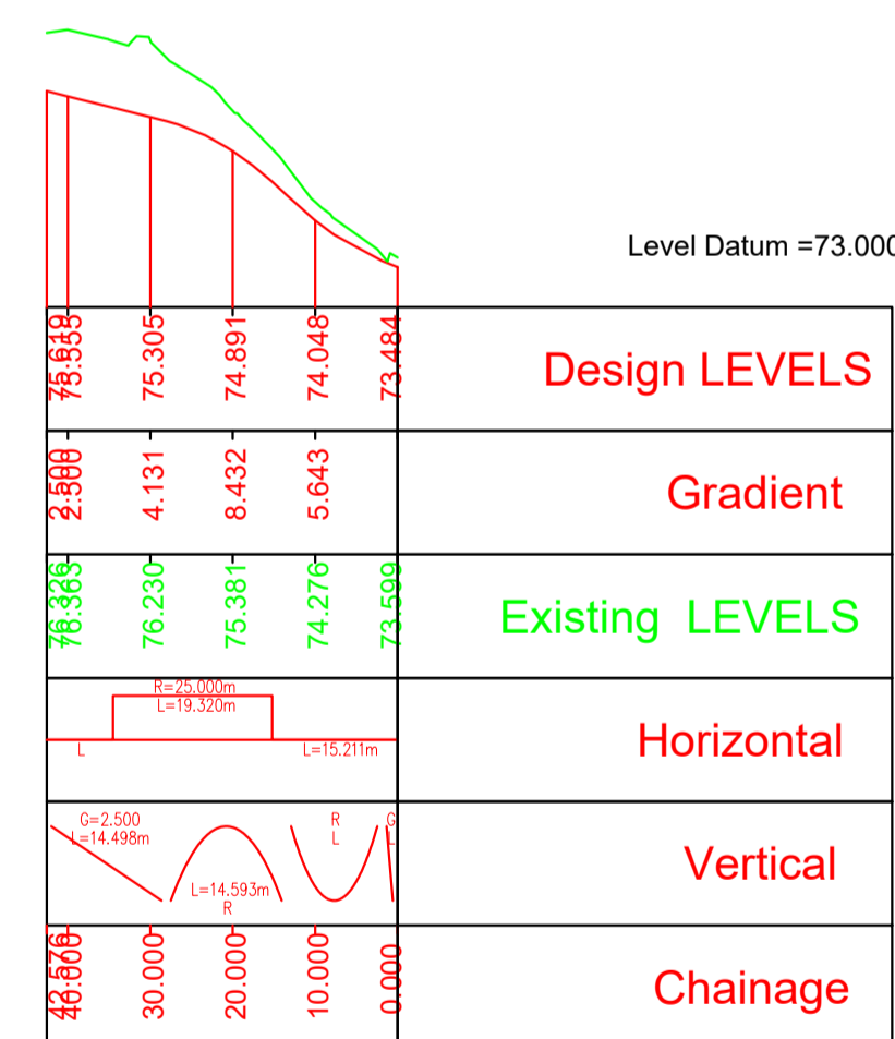
Long-section along Centreline of Direct Access No. 5 Common Farm Access
