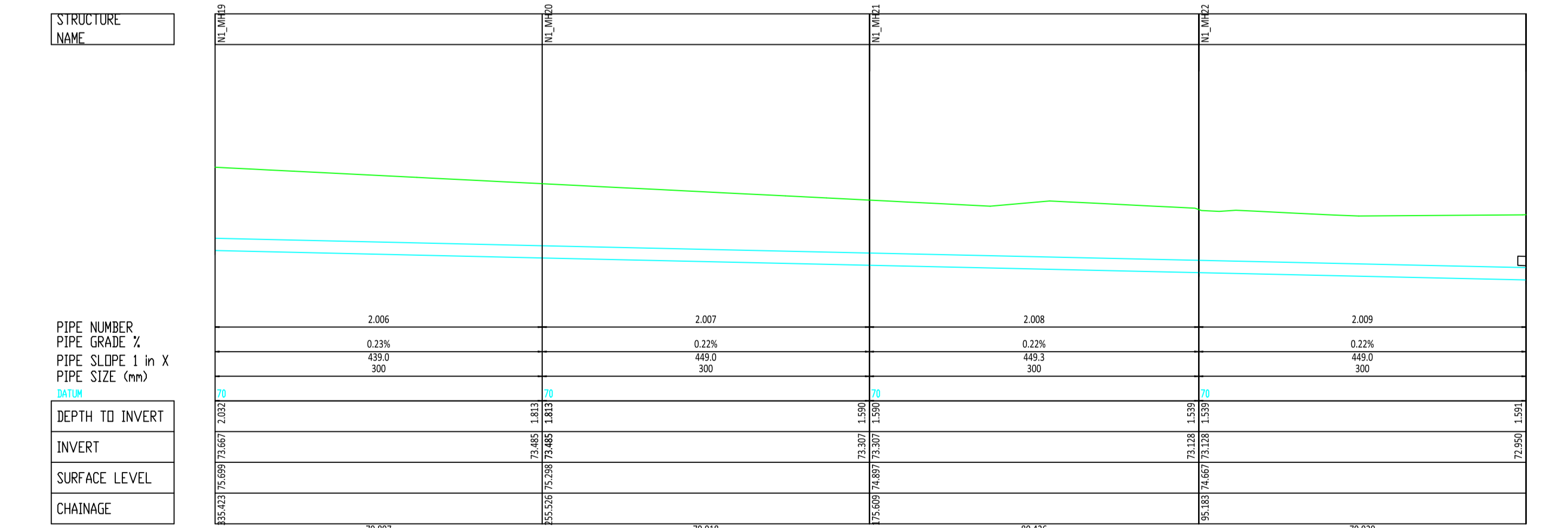
Longsection Drainage Network 1 (Pipe-run 2.006 to 2.010)
