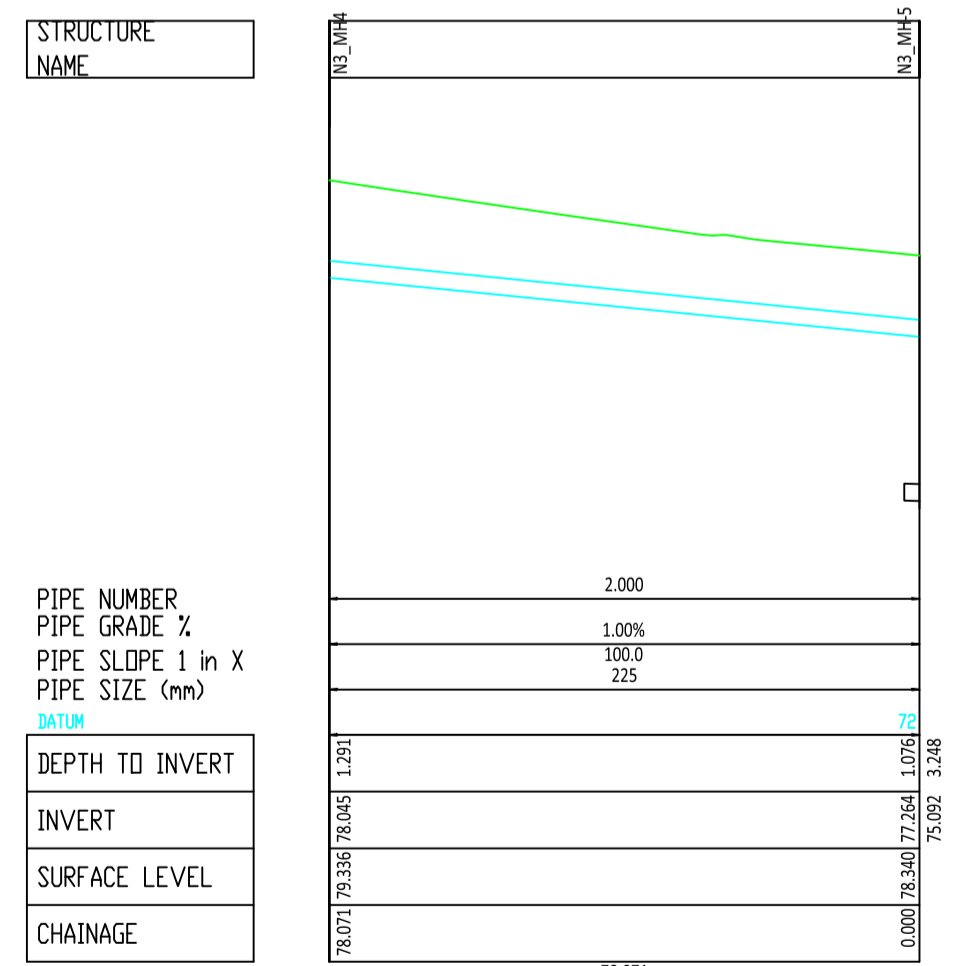
Longsection Drainage Network 3 (Pipe-run 2.000)
