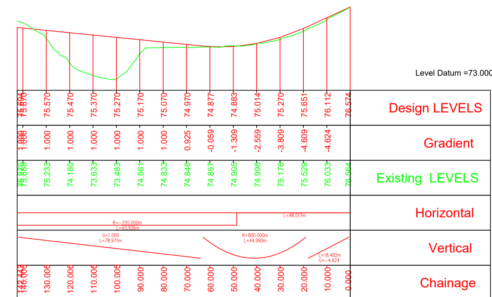
Long-section along Centreline of Direct Access No. 1 Local Road (L5833)
