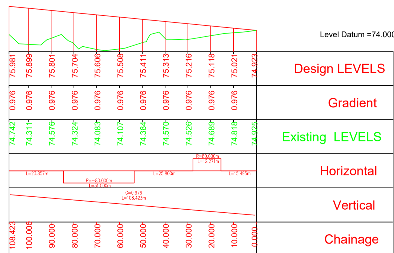
Long-section along Centreline of Direct Access No. 3 Public
