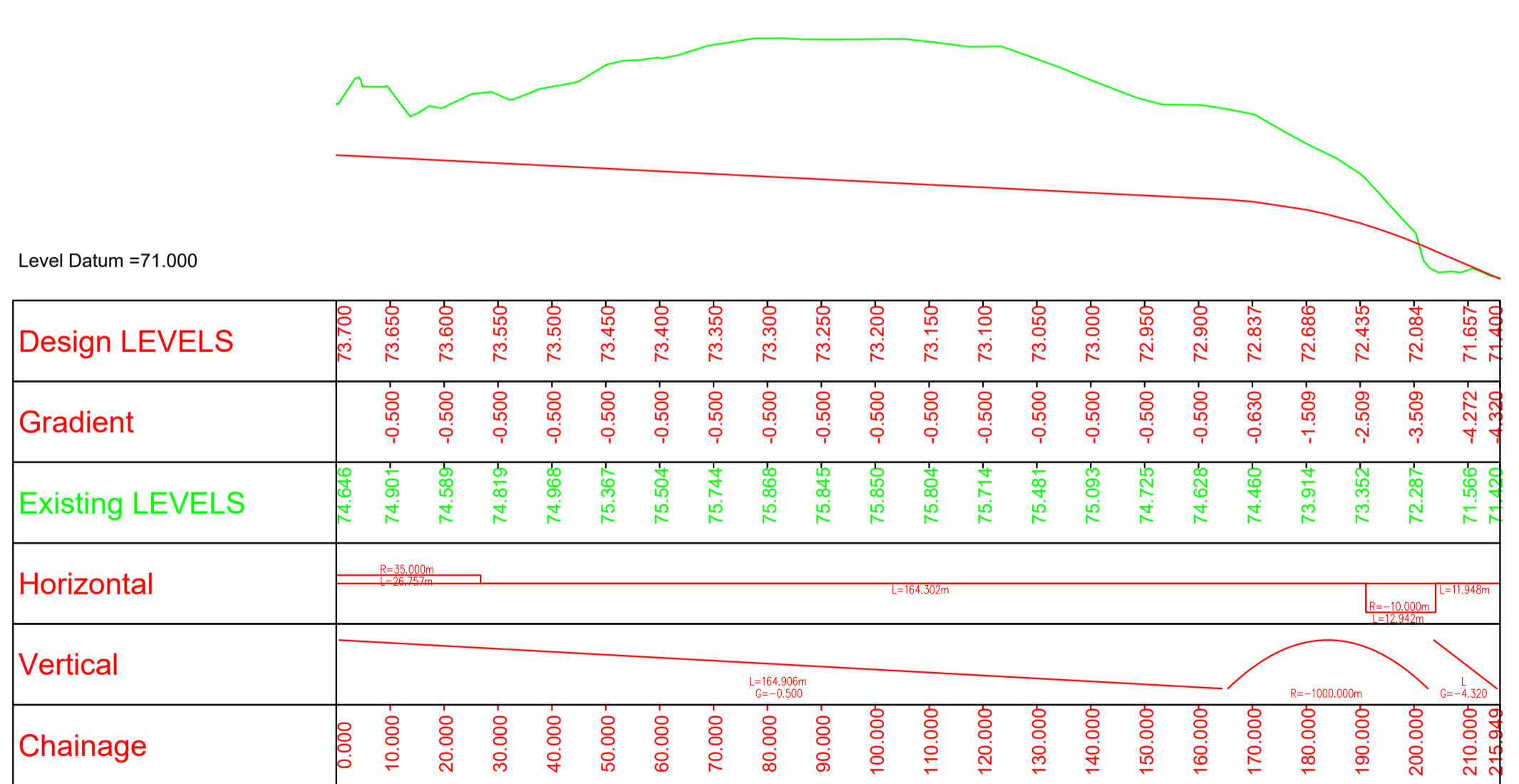
Long-section along Centreline of the Proposed Realigned Common Farm Access Road
