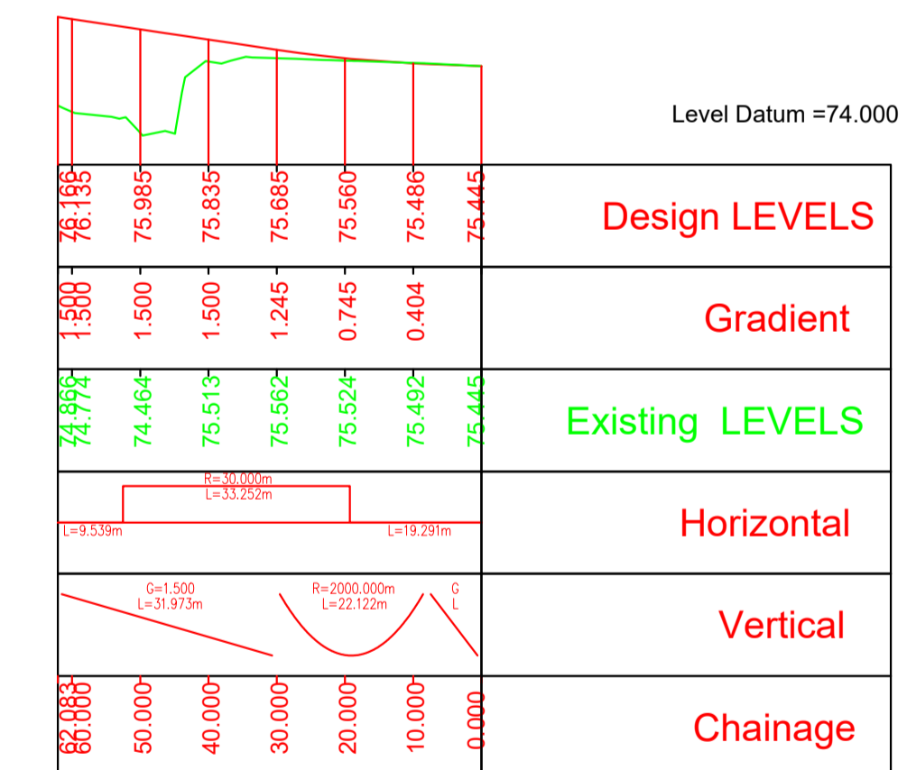
Long-section along Centreline of Direct Access No. 4 Public
