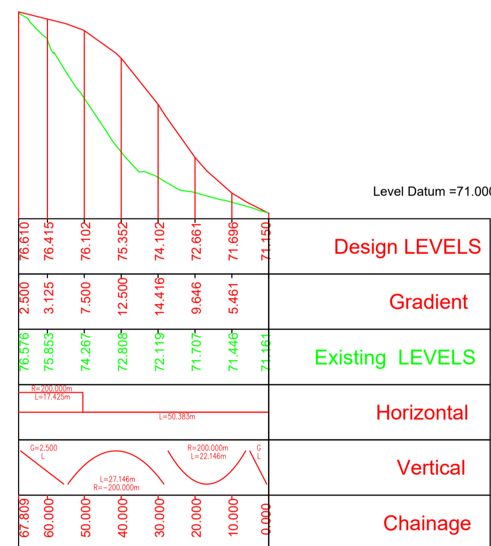
Long-section along Centreline of Direct Access No. 6 Common Field Access
