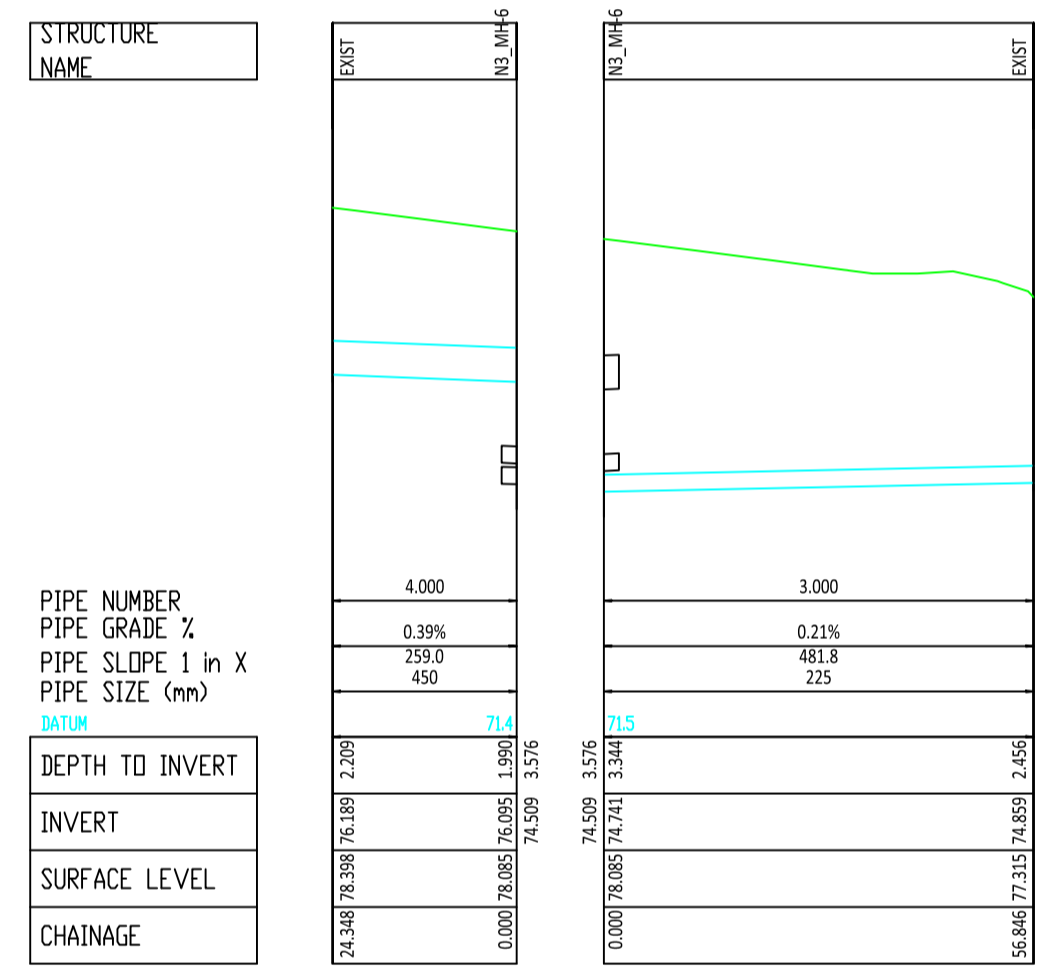
Longsection Drainage Network 3 (Pipe-run 3.000 & 4.000)
