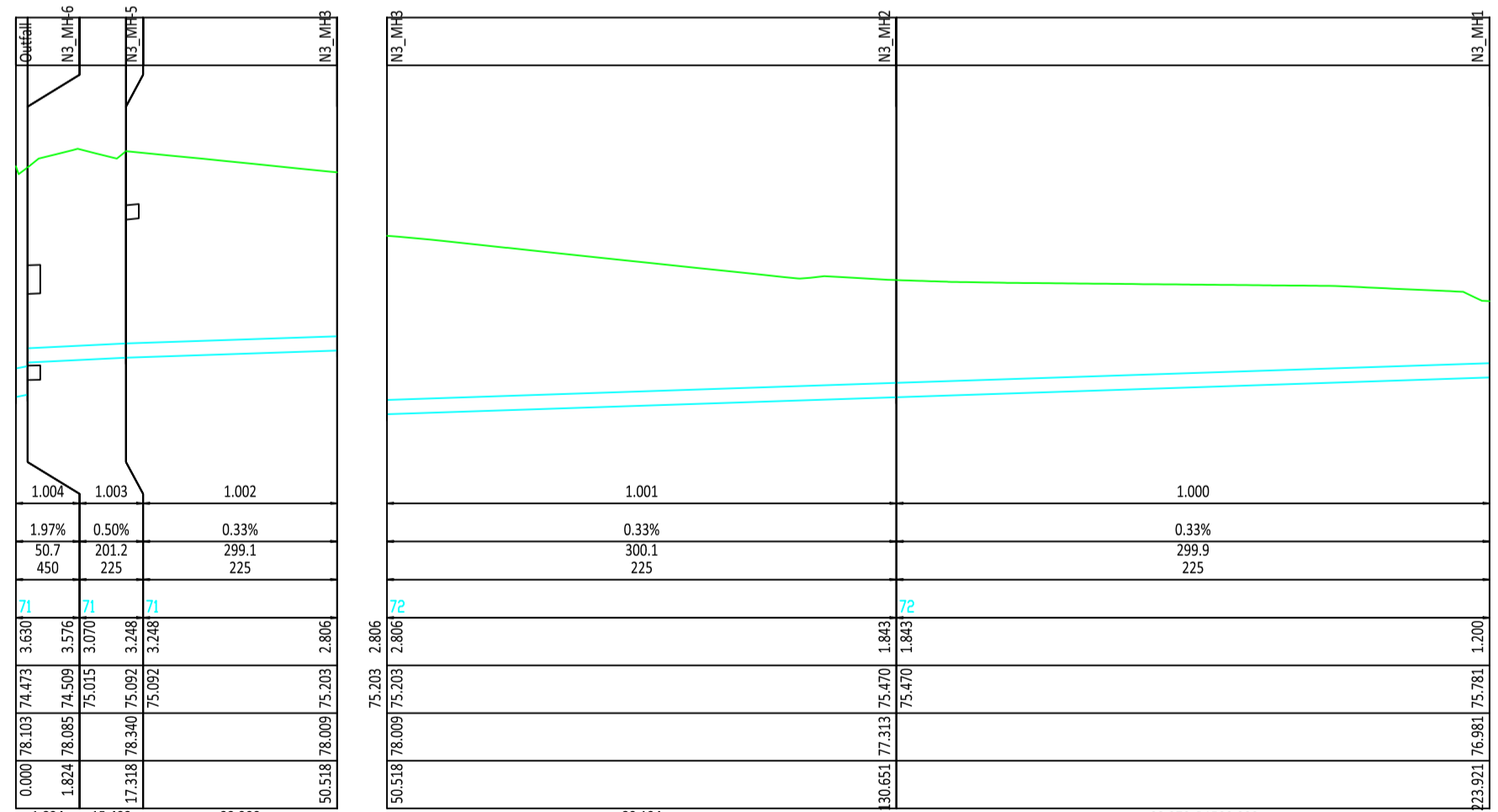
Longsection Drainage Network 3 (Pipe-run 1.000 to 1.004)
