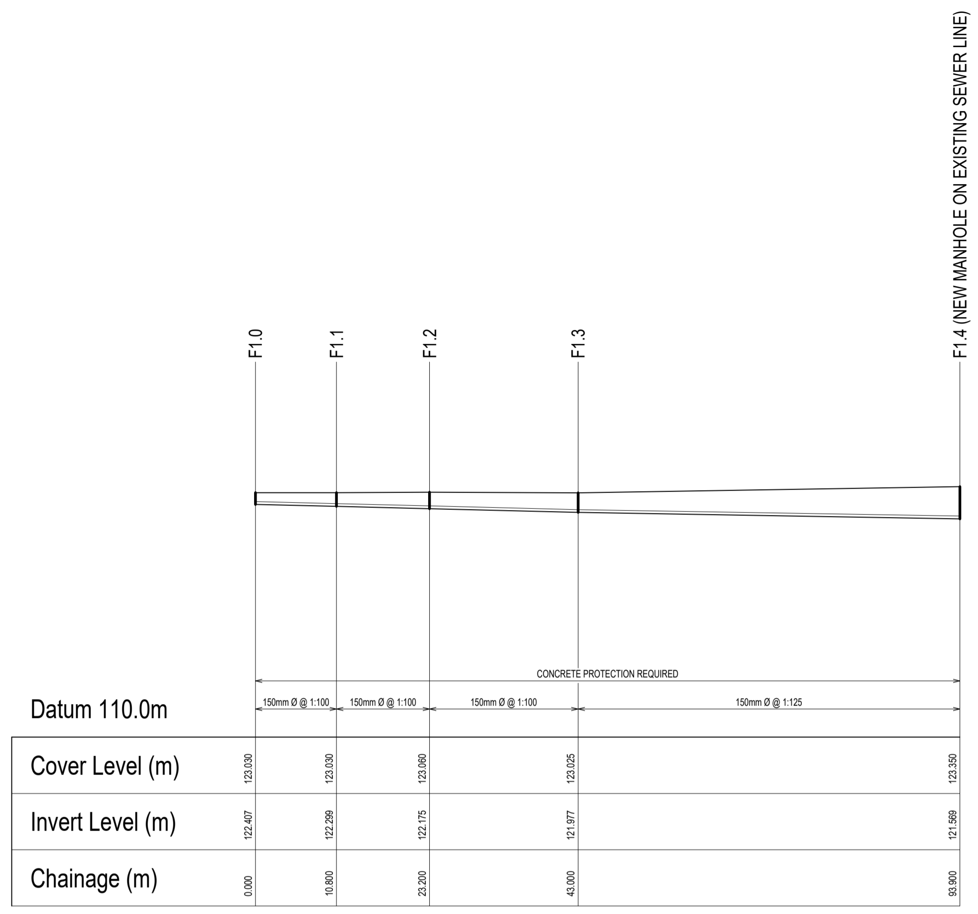
F1.0 - F1.4 (NEW MANHOLE ON EXISTING SEWER LINE) Scale: Horizontal 1:500, Vertical 1:100
