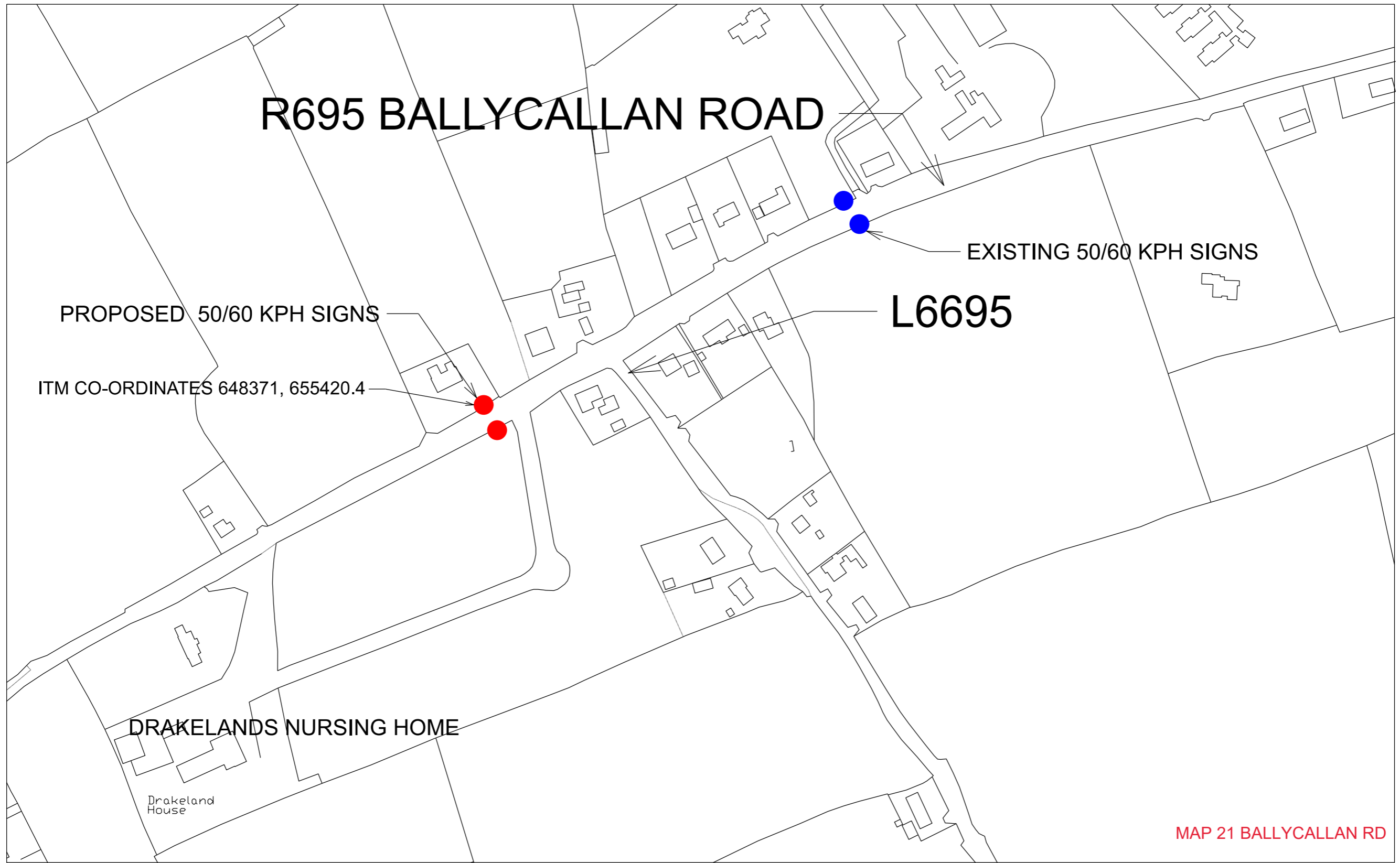
PROPOSED REVISED LOCATION OF 50/60 KPH SPEED LIMIT SIGN ON BALLYCALLAN ROAD
