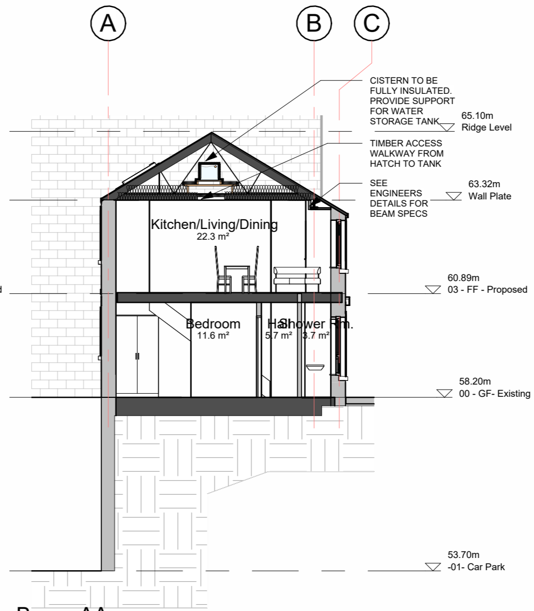
Beam AA
