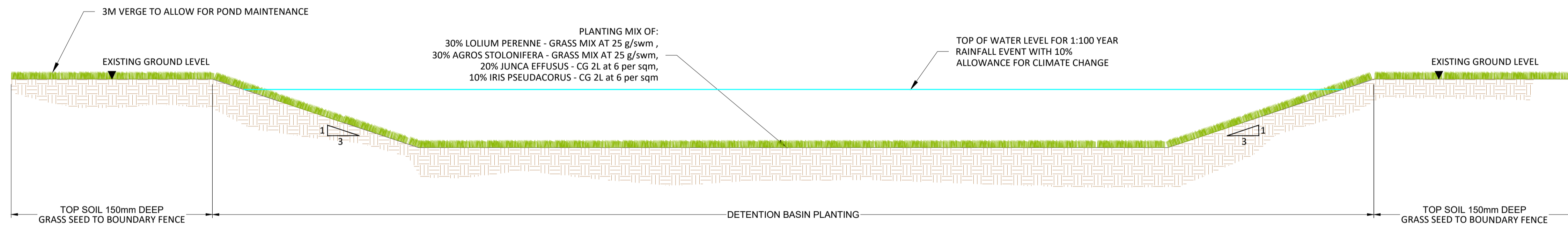
TYPICAL DETENTION BASIN CROSS SECTION
