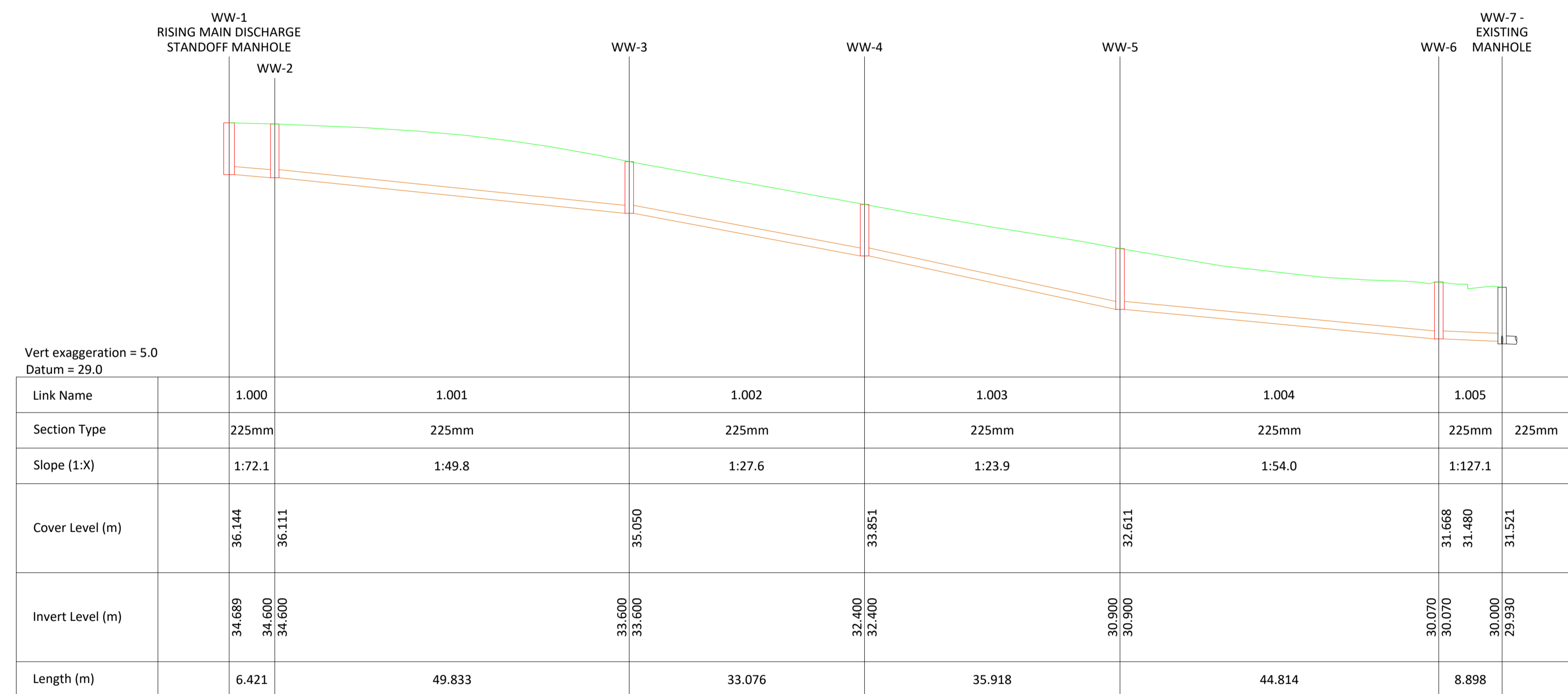
WASTEWATER NETWORK WW-1.000 - WW-1.005
