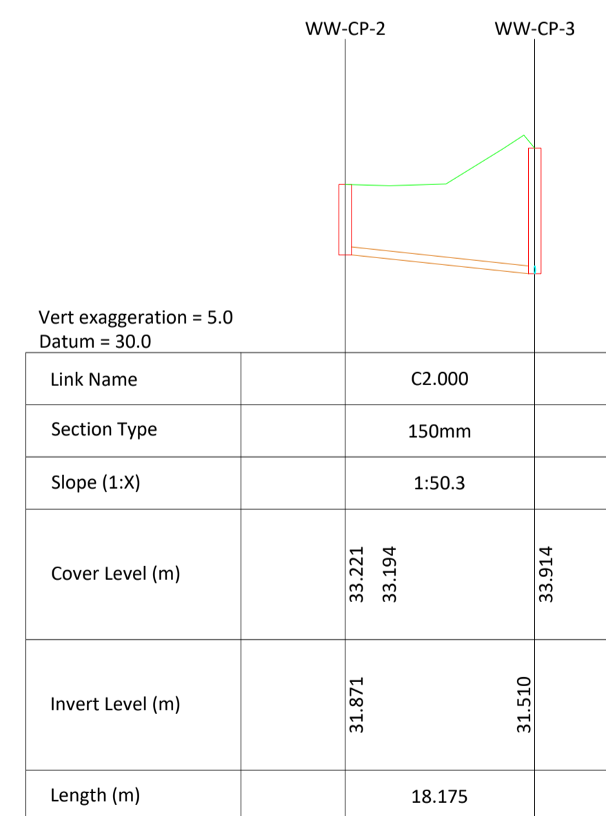
WASTEWATER NETWORK WW-CP-2.000
