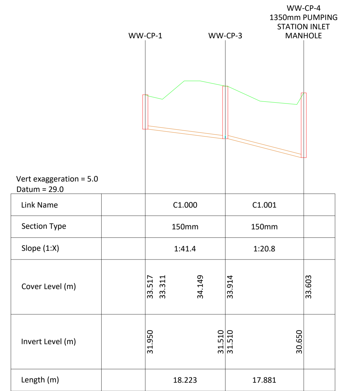
WASTEWATER NETWORK WW-CP-1.000 - WW-CP-1.001
