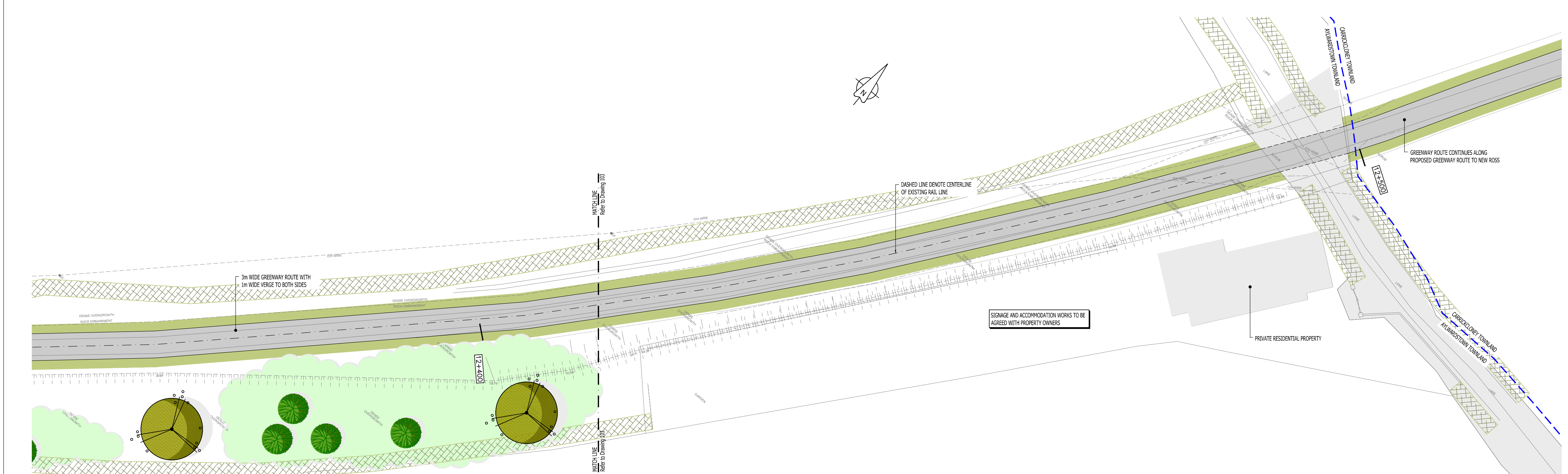
WATERFORD TO NEW ROSS GREENWAY (CHAINAGE 12.4km TO 12.5km)
