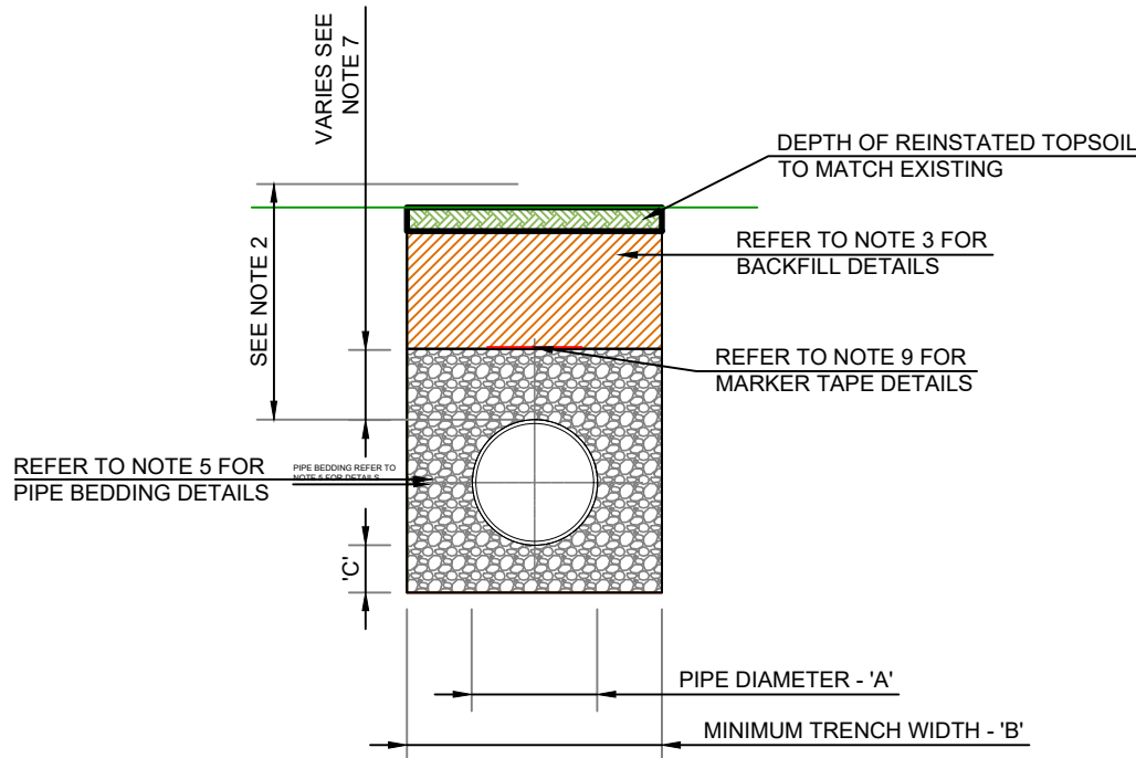
CROSS SECTION IN GRASSED AREAS
