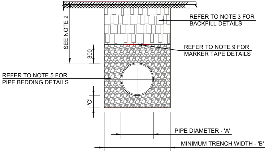
CROSS SECTION IN ROADS
