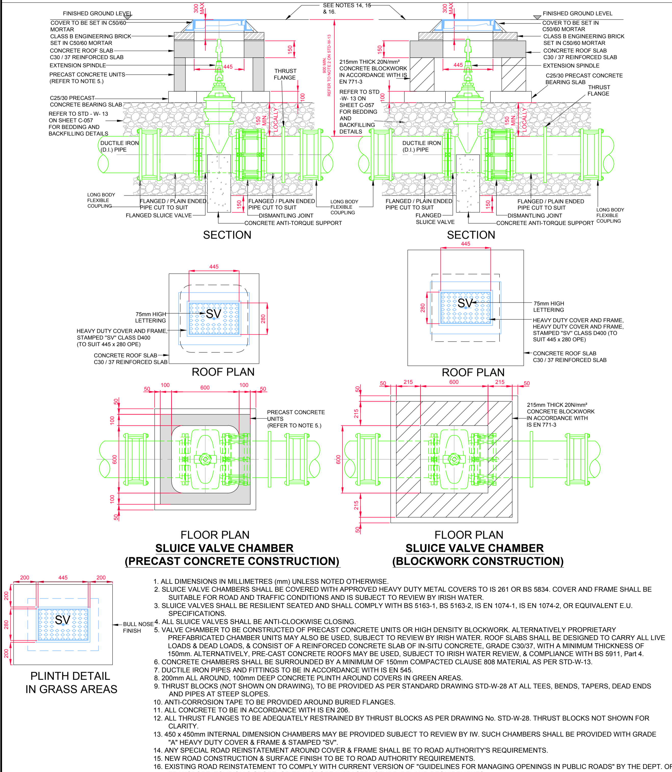
IRISH WATER - STANDARD DETAILS - WATER SLUCE VALVE FOR DUCTILE IRON (D.I.) PIPE (<350mm DIA.) (Sheet 1 of 2) - STD-W-14
