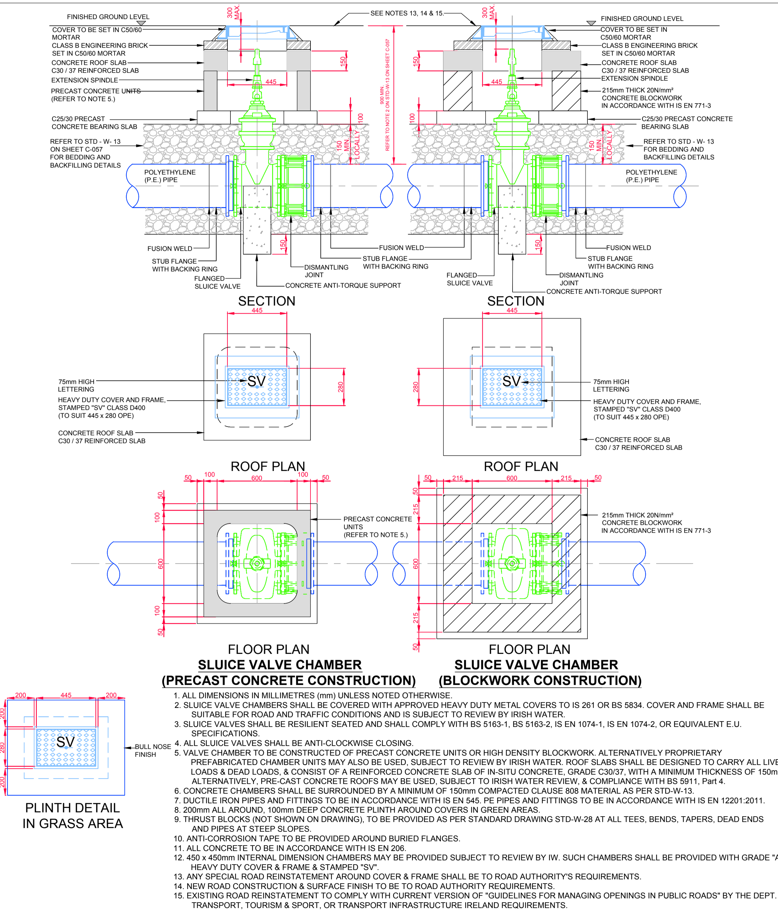
IRISH WATER - STANDARD DETAILS - WATER SLUCE VALVE FOR POLYETHYLENE (P.E.) PIPE (<350mm DIA.) (Sheet 2 of 2) - STD-W-15
