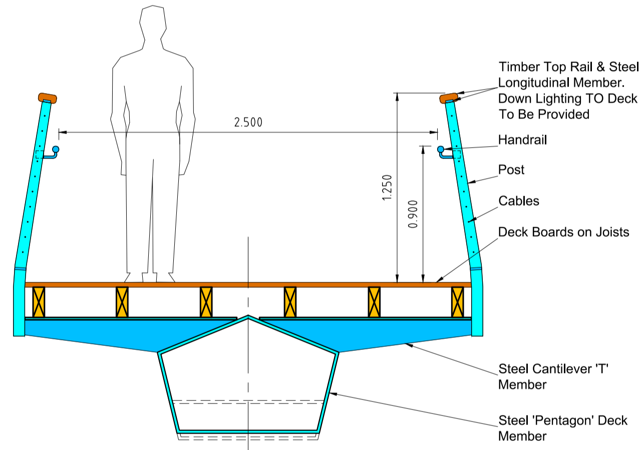
SECTION 2-2 [Scale 1 : 25] (PL0102-01)
