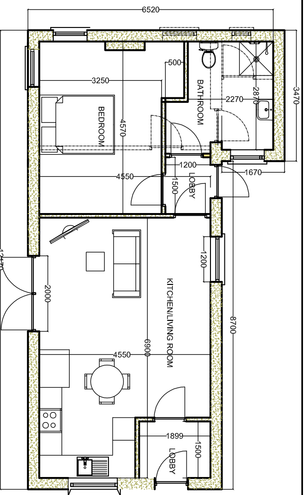
PROPOSED FLOOR LAYOUT AREA 58M 2 SCALE 1:100
