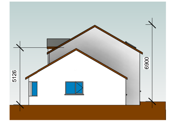
3 Side Elevation 1 1 : 200
