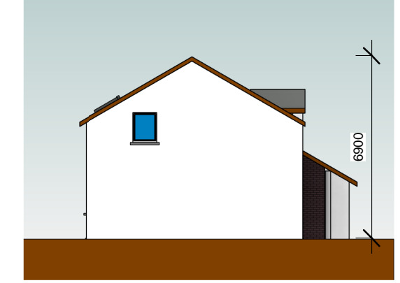
6 Side Elevation 2 1 : 200
