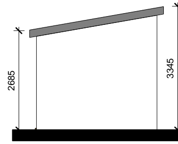
2 East/Side Elevation 1 : 100
