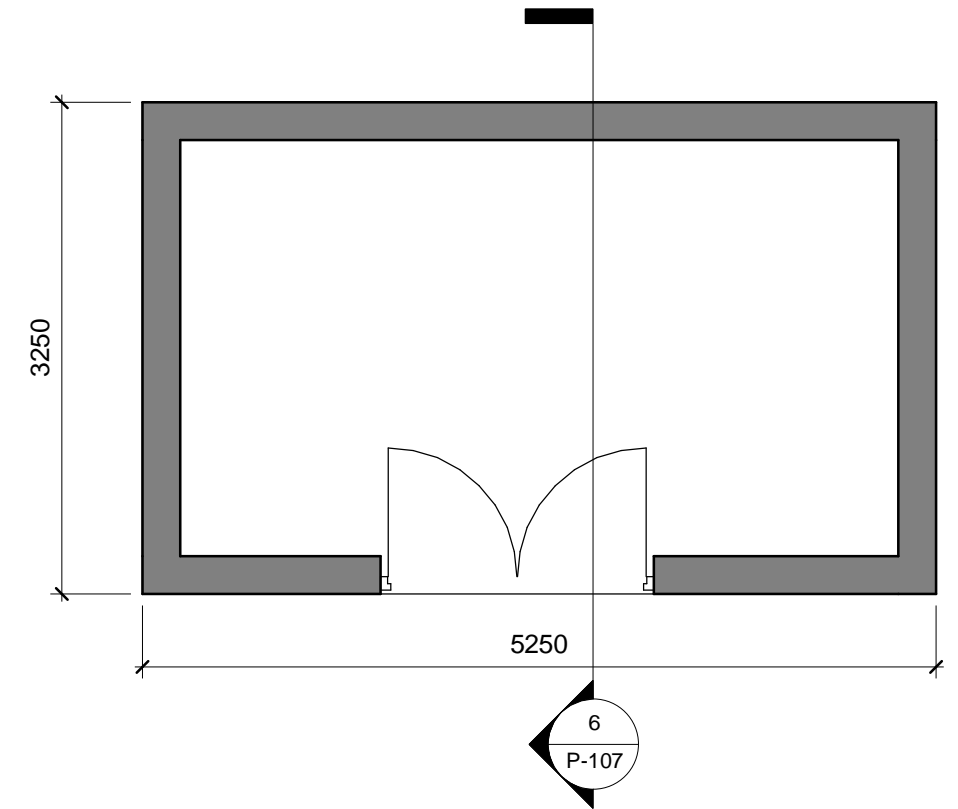
1 01-Floor Plan 1 : 50
