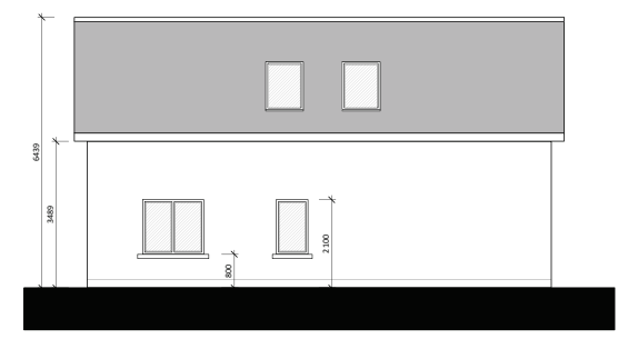
05 PROPOSED SIDE (NORTH) ELEVATION 1:100 @ A1
