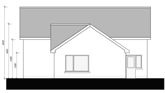
01 PROPOSED SIDE (SOUTH) ELEVATION 1:100 @ A1
