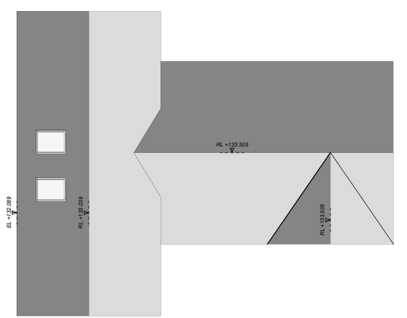
09 PROPOSED ROOF PLAN 1:100 @ A1
