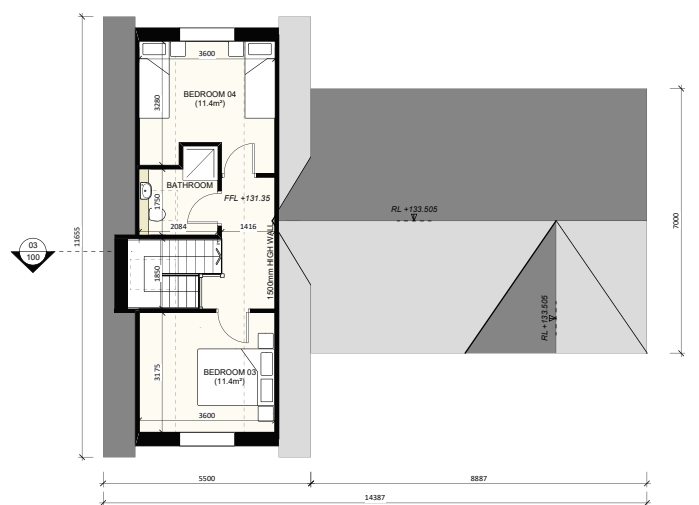
08 PROPOSED 1st FLOOR PLAN 1:100 @ A1
