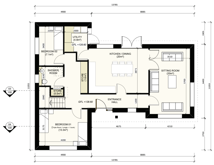
07 PROPOSED GROUND FLOOR PLAN 1:100 @ A1
