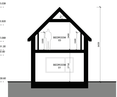
04 PROPOSED CROSS SECTION 1:100 @ A1
